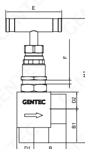
Angle Pattern
