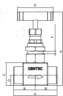
Straight Pattern
