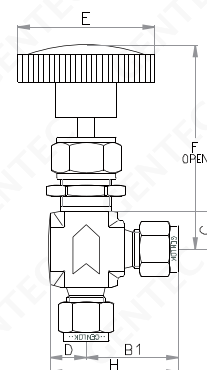
Angle Pattern
